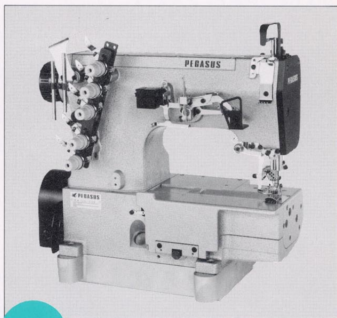
A Short-Bed Interlock Machine For Covering Operations
